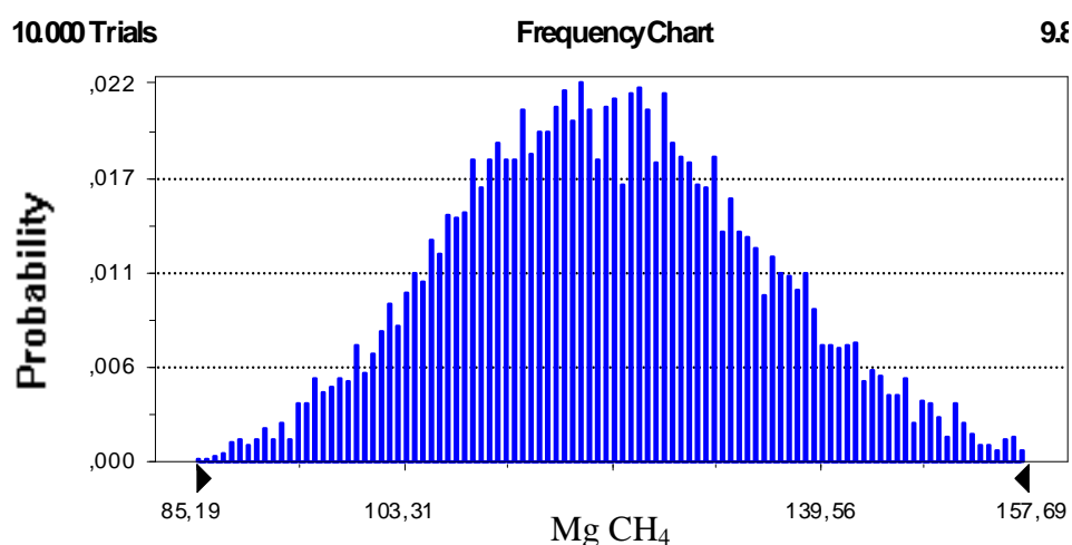
Figure A1.11 Probability density function resulting from Montecarlo analysis for CH 4 emissions from enteric fermentation, year 2010
