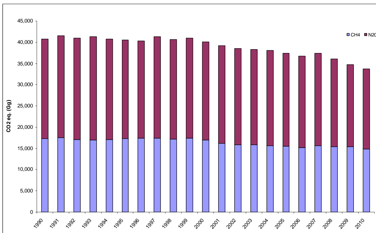
Figure 6.1 Trend of GHG emissions for the agriculture sector from 1990 to 2010 (Gg CO 2 eq.)
