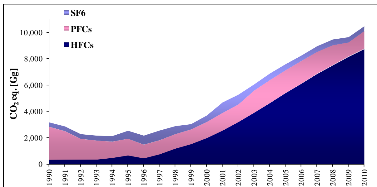
Figure 2.7 National emissions of fluorinated gases by sector from 1990 to 2010 (Gg CO 2 eq.)
