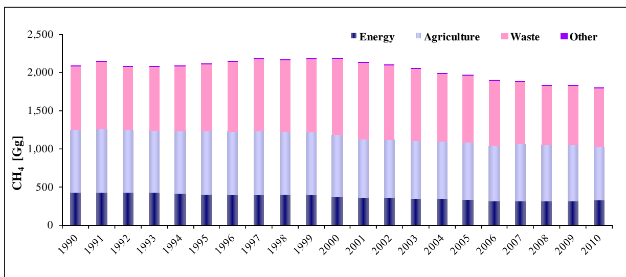
Figure 2.5 National CH 4 emissions by sector from 1990 to 2010 (Gg)
