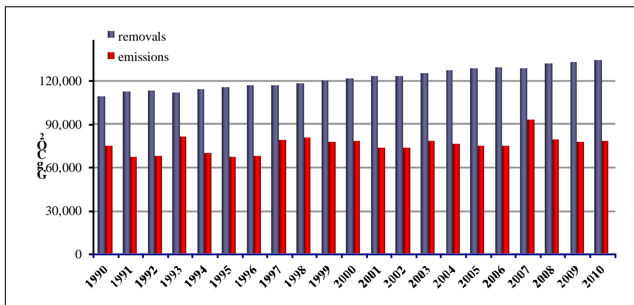
Figure 7.2 CO 2 removals and emissions in LULUCF sector in the period 1990-2010 [Gg CO 2 ]
