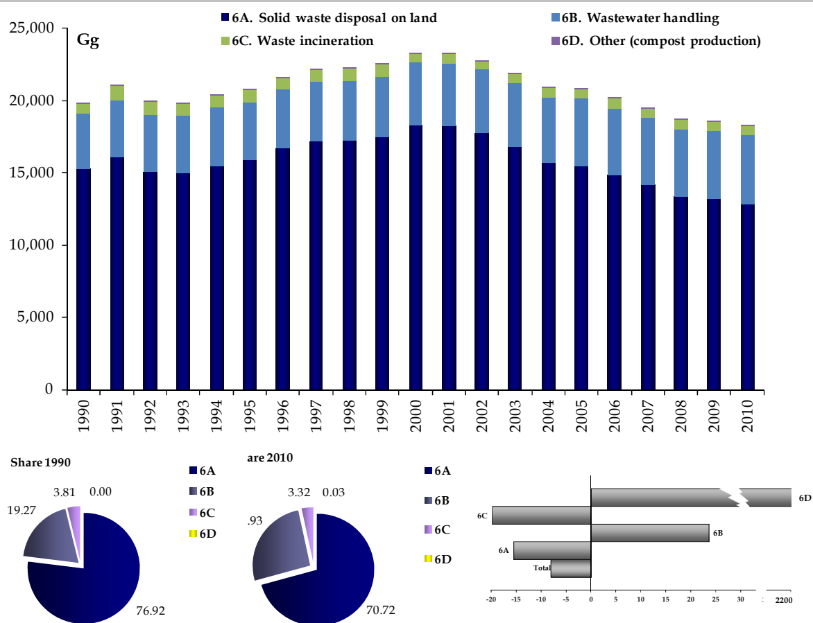
Figure 2.13 Trend of total emissions from the waste sector (1990-2010) (Gg CO 2 eq.)
