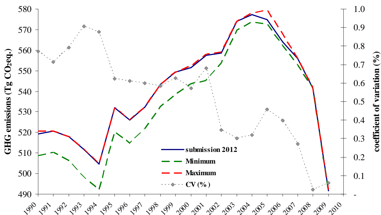
Figure 9.1 Range of national GHG emissions (Tg CO 2 eq.) in the 2001-2012 submissions and coefficient of variation (%)
