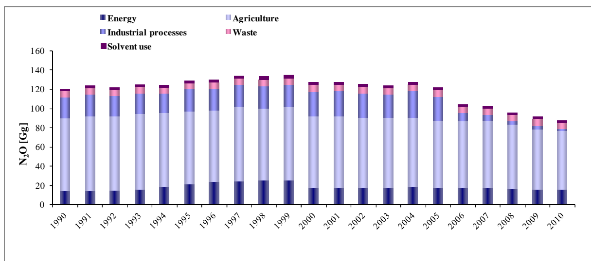
Figure 2.6 National N 2 O emissions by sector from 1990 to 2010 (Gg)
