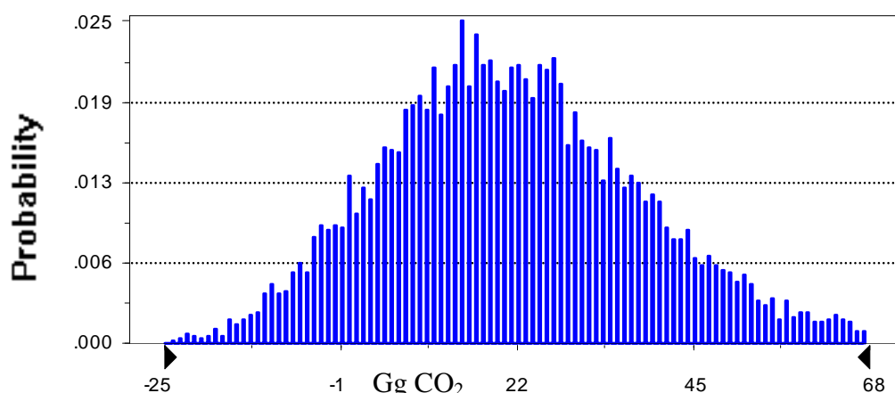
Figure A1.13 Probability density function resulting from Montecarlo analysis for the Land converting to Forest Land, year 2009
