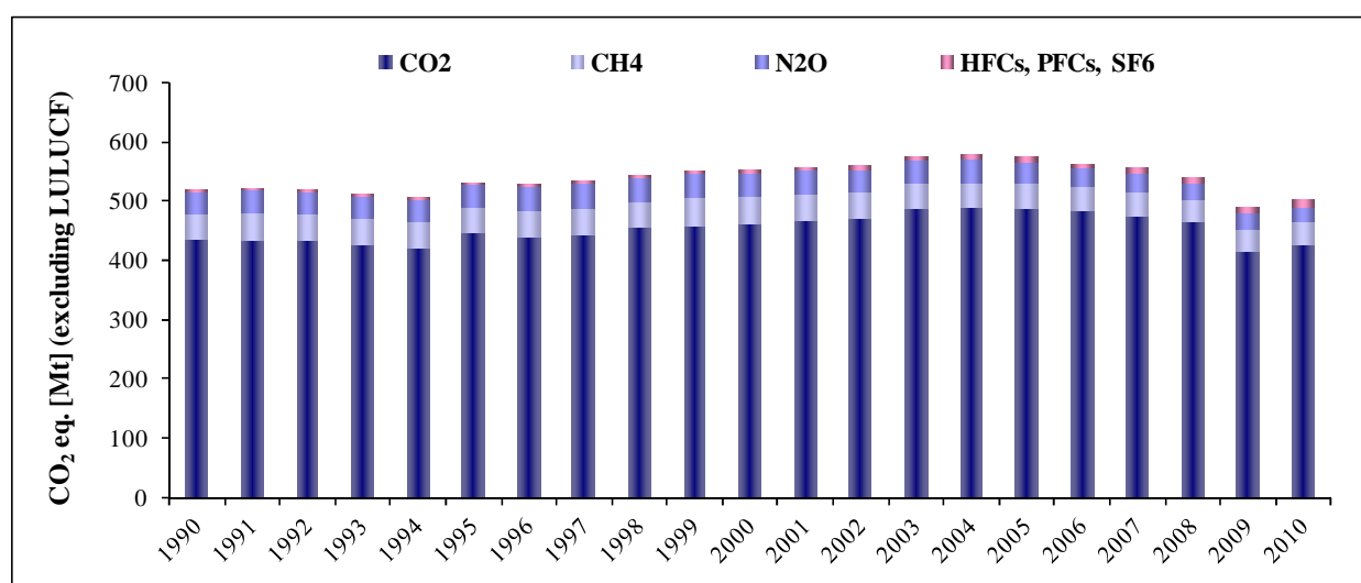
Figure 2.1 National greenhouse gas emissions from 1990 to 2010 (without LULUCF) (Mt CO 2 eq.)
