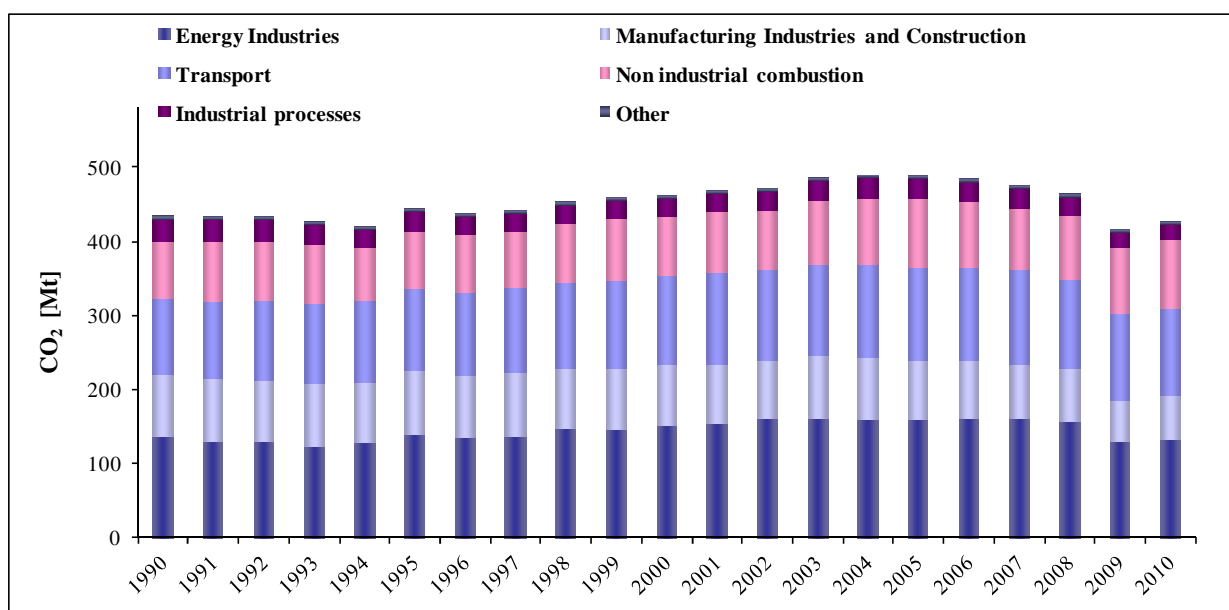
Figure 2.3 National CO 2 emissions by sector from 1990 to 2010 (Mt)
