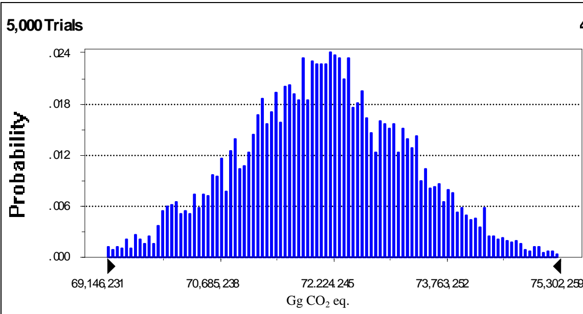
Figure A1.1 Probability density function result combustion of liquid fuels, year 2009
