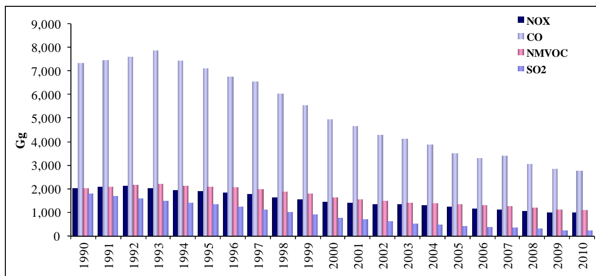
Figure 2.14 Trend of total emissions for indirect greenhouse gases and SO 2 (1990-2010) (Gg)
