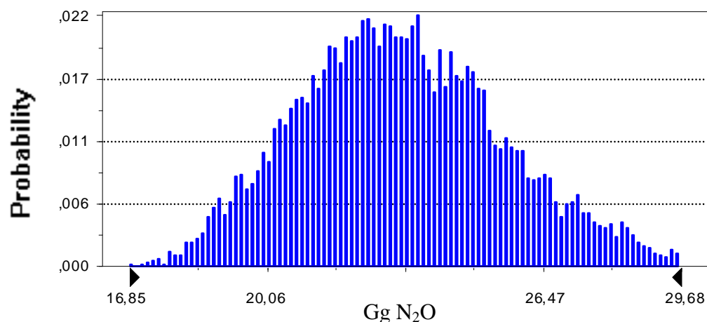
Figure A1.8 Probability density function resulting from Monte Carlo analysis for Direct N 2 O Agriculture soils emissions, year 2010
