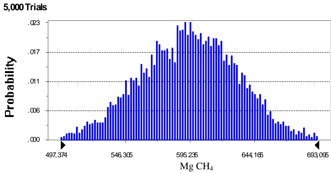
Figure A1.19 Probability density function resulting from Montecarlo analysis for the Solis waste disposal on land category, year 2009
