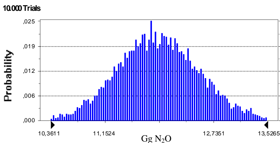
Figure A1.10 Probability density function resulting from Montecarlo analysis for N 2 O emissions from Manure management, year 2010
