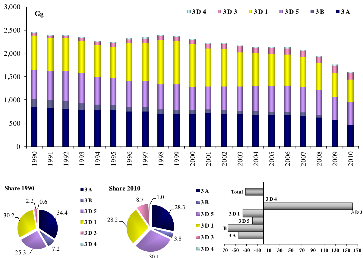
Figure 2.10 Trend of total emissions from the solvent and other product use sector (1990-2010) (Gg CO 2 eq.)
