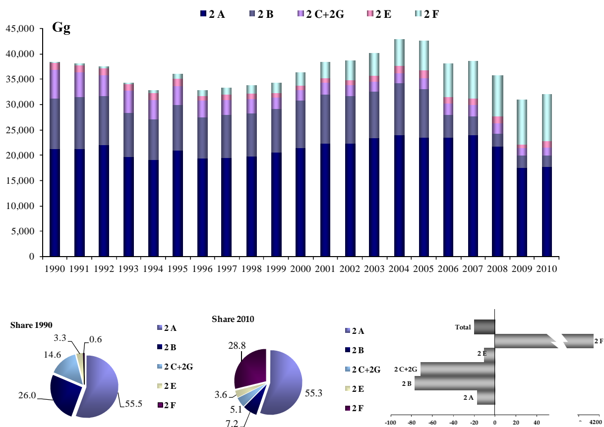
Figure 2.9 Trend of total emissions from the industrial processes sector (1990-2010) (Gg CO 2 eq.)
