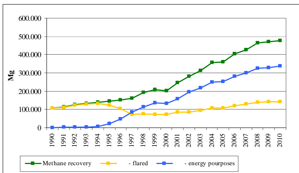
Figure 8.2 Methane recovery distinguished in flared amount and energy purposes (Mg)
