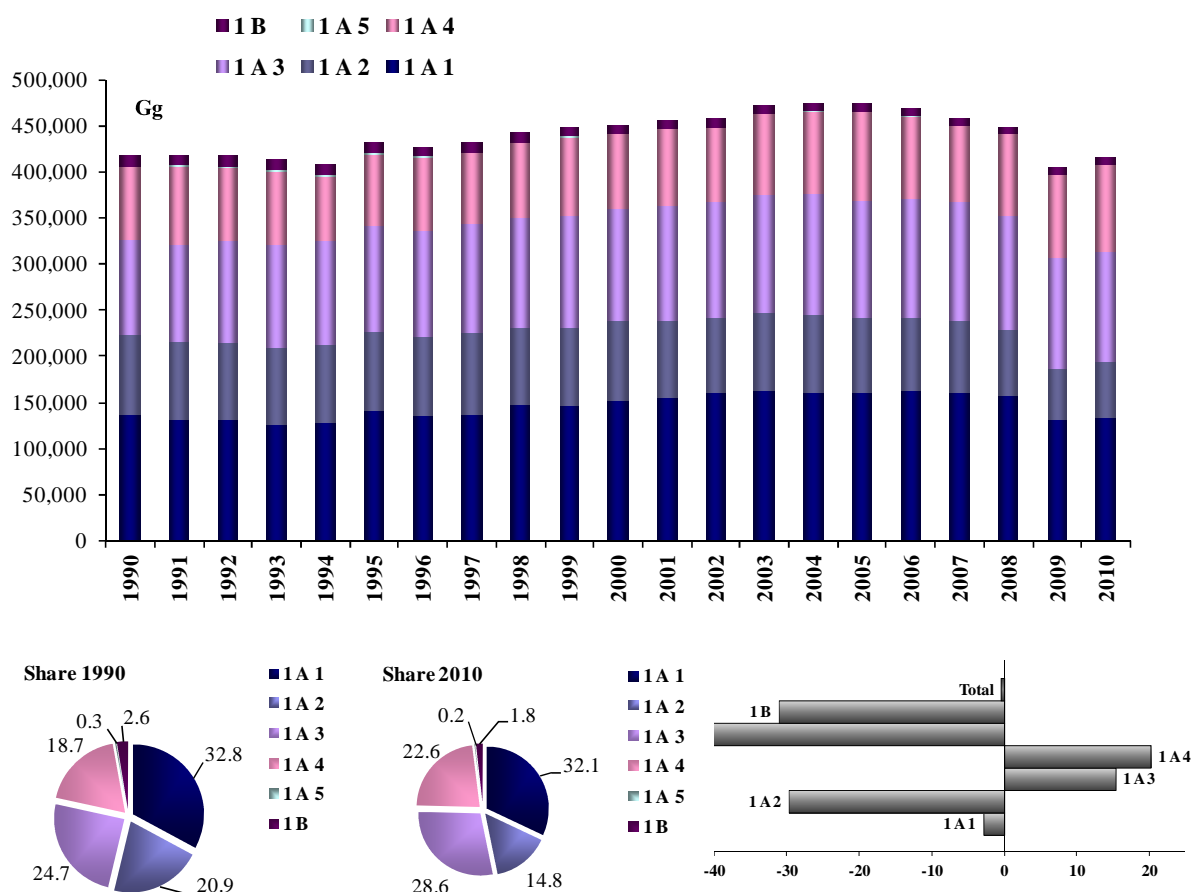
Figure 2.8 Trend of total emissions from the energy sector (1990-2010) (Gg CO 2 eq.)
