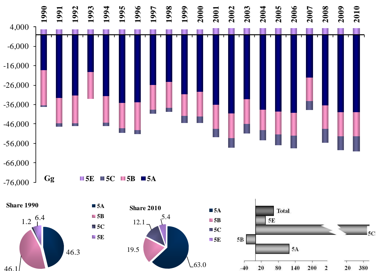
Figure 2.12 Trend of total emissions and removals from the LULUCF sector (1990-2010) (Gg CO 2 eq.)
