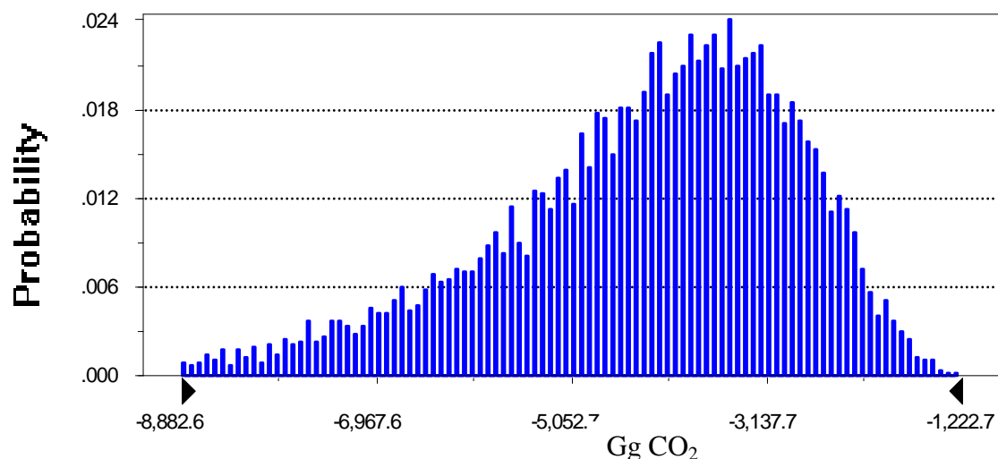
Figure A1.18 Probability density function resulting from Montecarlo analysis for the CO 2 emissions from Land converting to Settlements, year 2009
