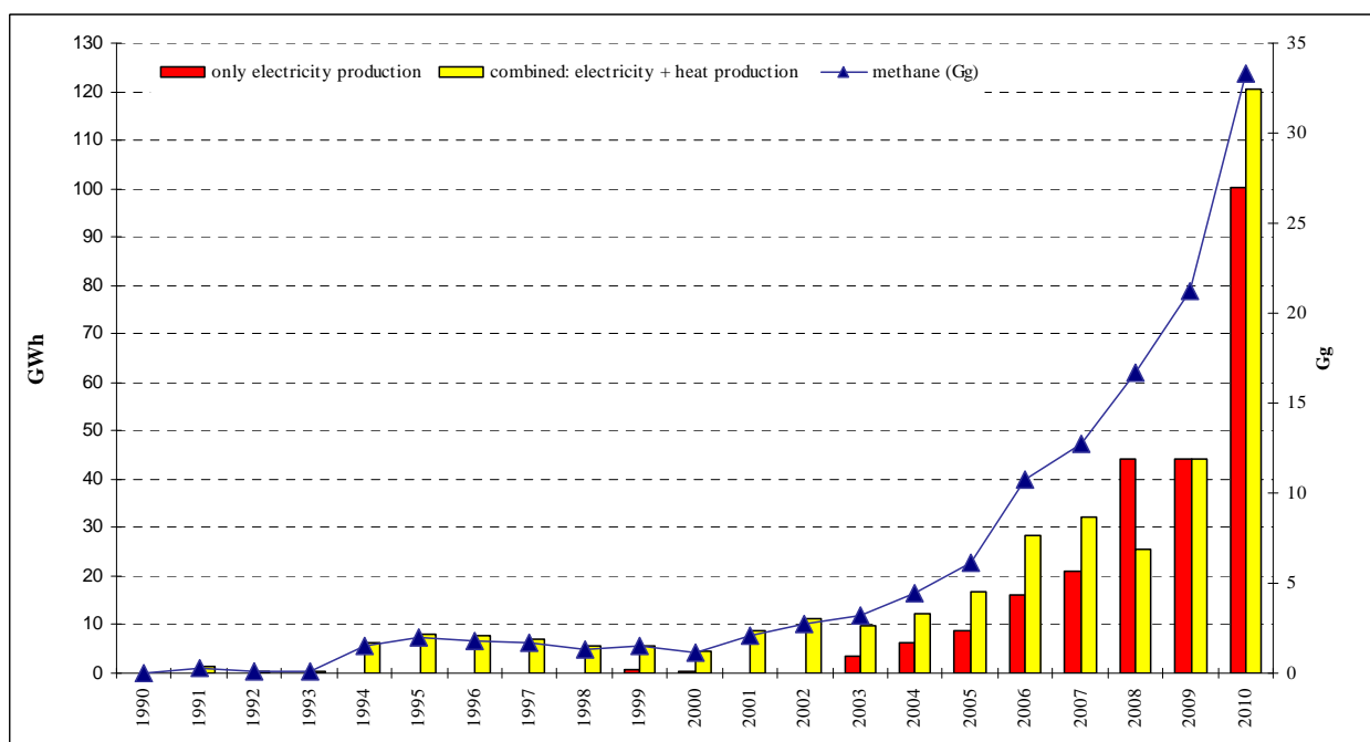
Figure A7.1 Time series of gross production of biogas from animal manure
