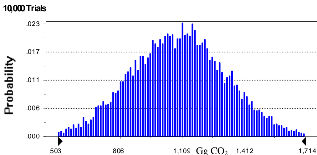
Figure A1.12 Probability density function resulting from Montecarlo analysis for the CO 2 emissions and removals from Forest Land remaining Forest Land category, year 2009
