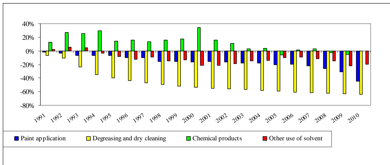
Figure 5.1 Trend of NMVOC emissions from 1991 to 2010 as compared to 1990
