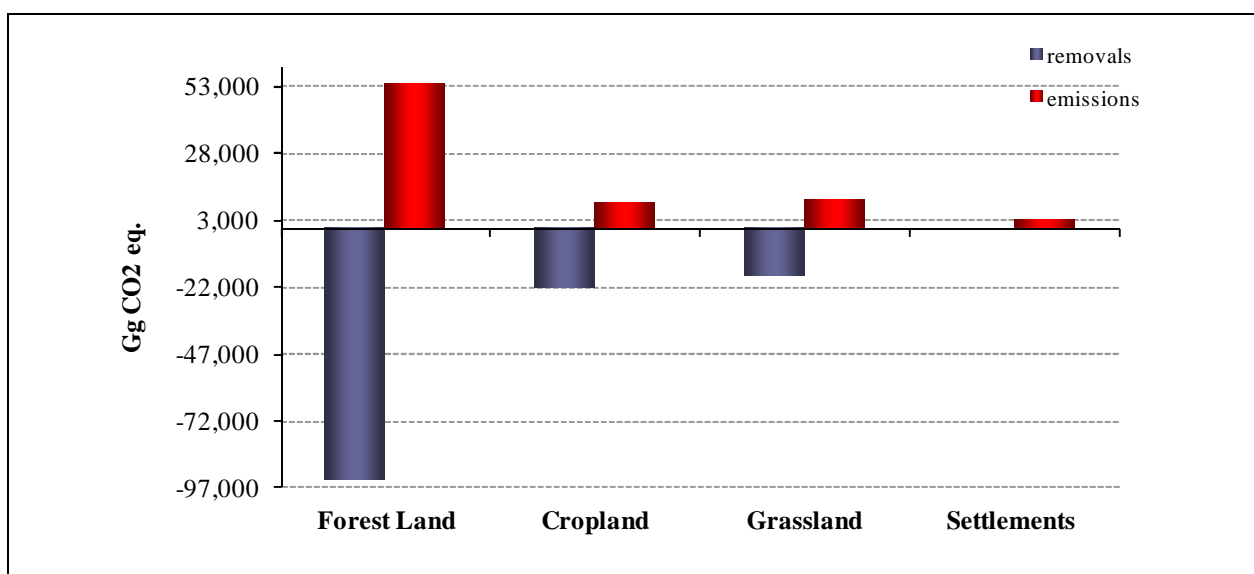
Figure 7.1 Greenhouse gas removals and emissions in LULUCF sector in 2010 [Gg CO 2 eq.]
