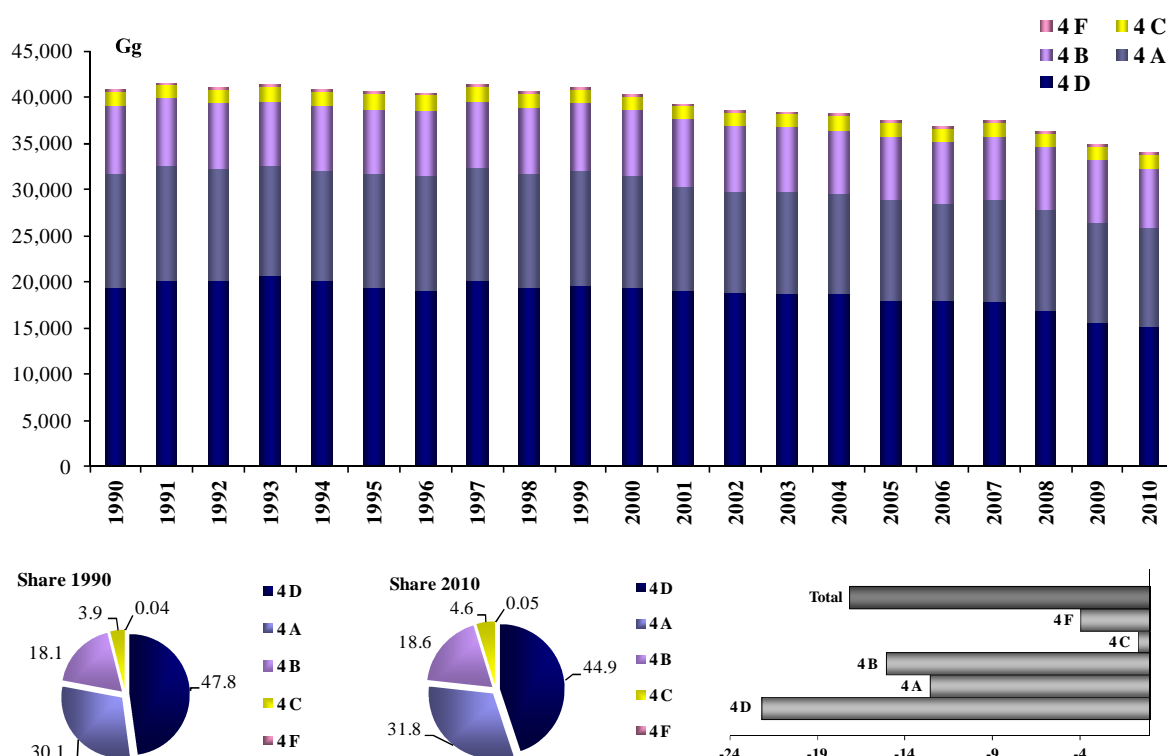
Figure 2.11 Trend of total emissions from the agriculture sector (1990-2010) (Gg CO 2 eq.)
