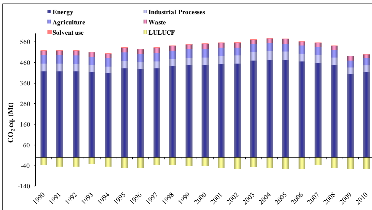
Figure 2.2 Greenhouse gas emissions and removals from 1990 to 2010 by sector (Mt CO 2 eq.)
